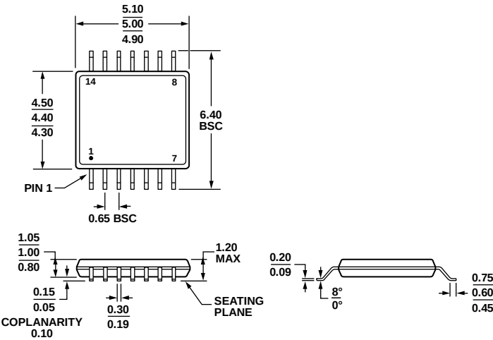
COMPLIANT TO JEDEC STANDARDS MO-153-AB-1 Figure 66. 14-Lead Thin Shrink Small Outline Package [TSSOP] (RU-14) Dimensions shown in millimeters
