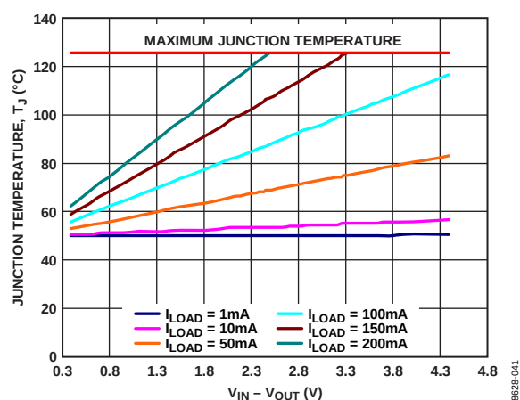
Figure 43. 500 mm² of PCB Copper, WLCSP, T_A = 85^\circ\text{C}
