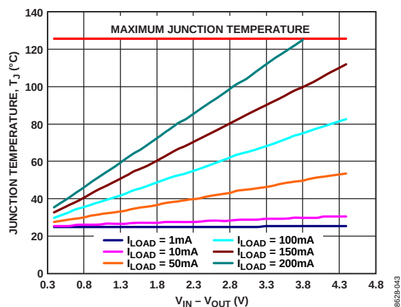
Figure 45. 500 mm² of PCB Copper, TSOT, T_A = 25^\circ\text{C}
