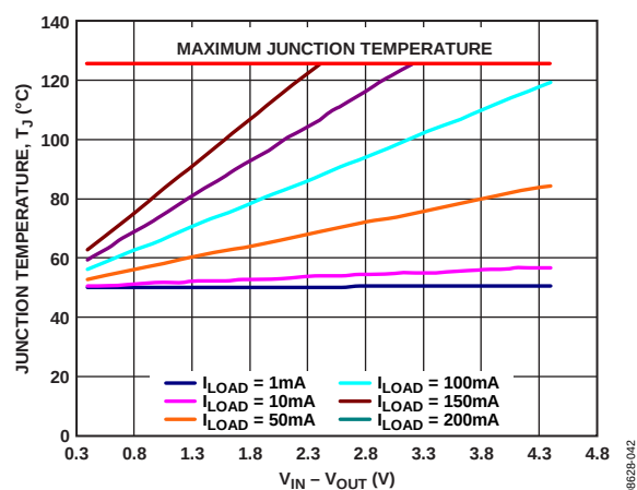
Figure 44. 100 mm² of PCB Copper, WLCSP, T_A = 50^\circ\text{C}
