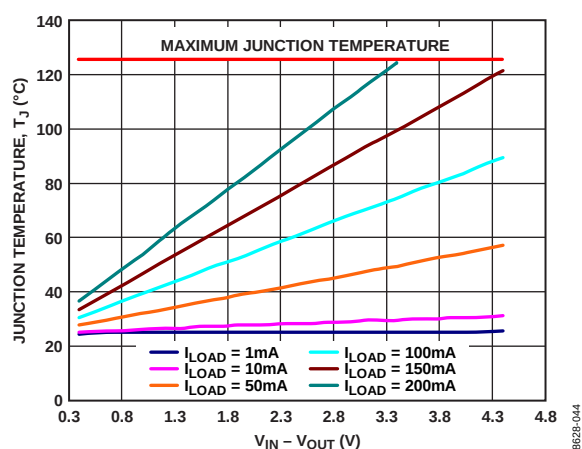
Figure 46. 100 mm² of PCB Copper, TSOT, T_A = 25^\circ\text{C}
