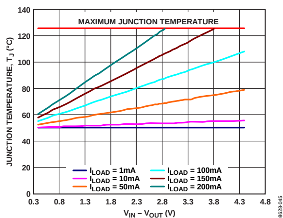
Figure 47. 500 mm² of PCB Copper, TSOT, T_A = 50^\circ\text{C}
