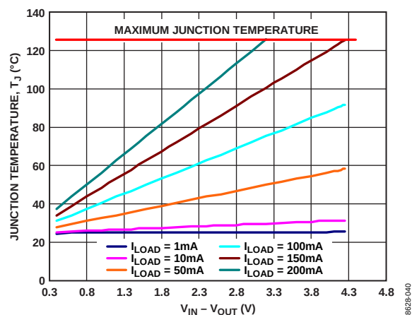
Figure 42. 100 mm² of PCB Copper, WLCSP, T_A = 50^\circ\text{C}
