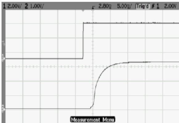
Fig.65 AVO50-48S3V3 typical start-up from power on
