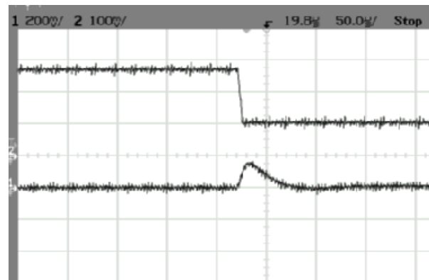
Fig.41 AVO50-48S3V3 typical transient response to step increase in load from 50% to 75% of full load, room temperature, 48Vdc input ( \Delta I_o/\Delta t = 1A/1\mu s )
