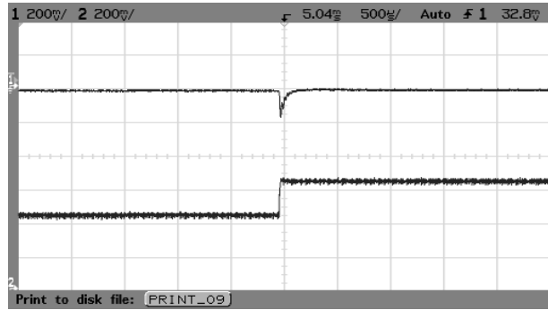
Fig.49 AVO50-48S12 typical transient response to step increase in load from 50% to 75% of full load, room temperature, 48Vdc input ( \Delta I_o/\Delta t = 1A/1\mu s )
