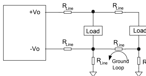
Fig.77 Ground loops
