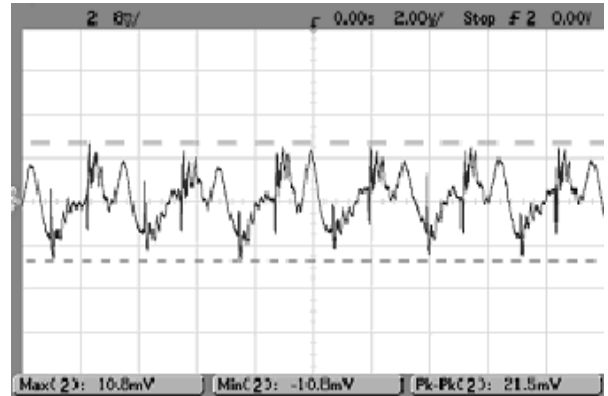
Fig.55 Typical output ripple voltage of AVO50-48S05 room temperature, I_o = I_{o,max}
