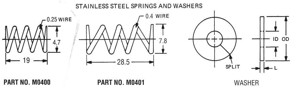
WASHER SIZES
