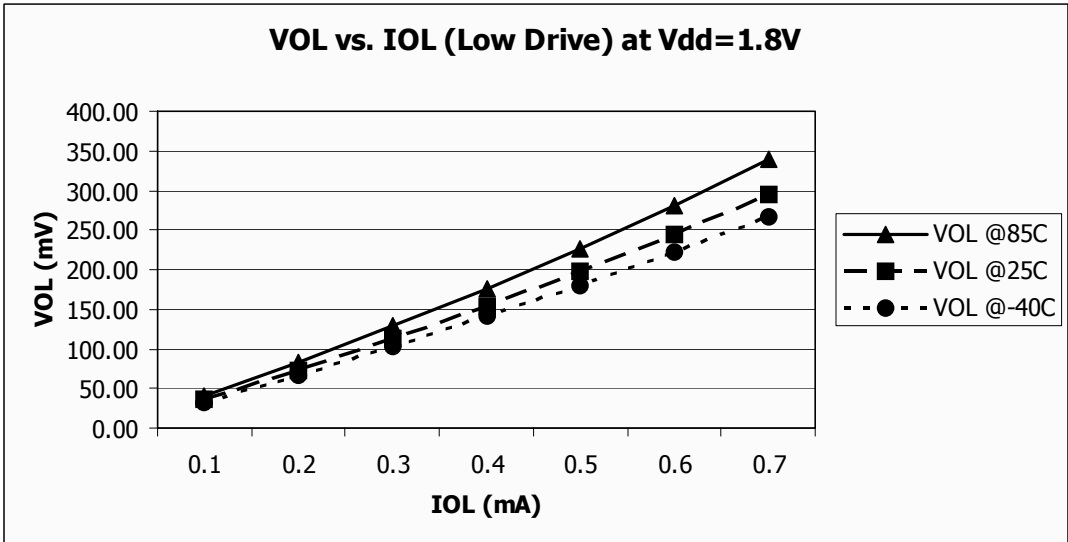
Figure 17. Typical V_{OL} vs. I_{OL} V_{DD} = 1.8\text{ V} (Low Drive)
