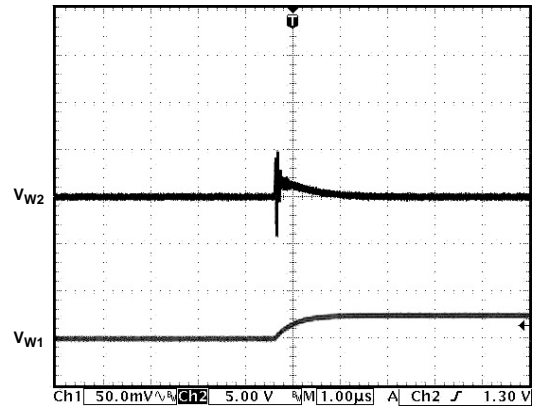
Figure 27. Analog Crosstalk
