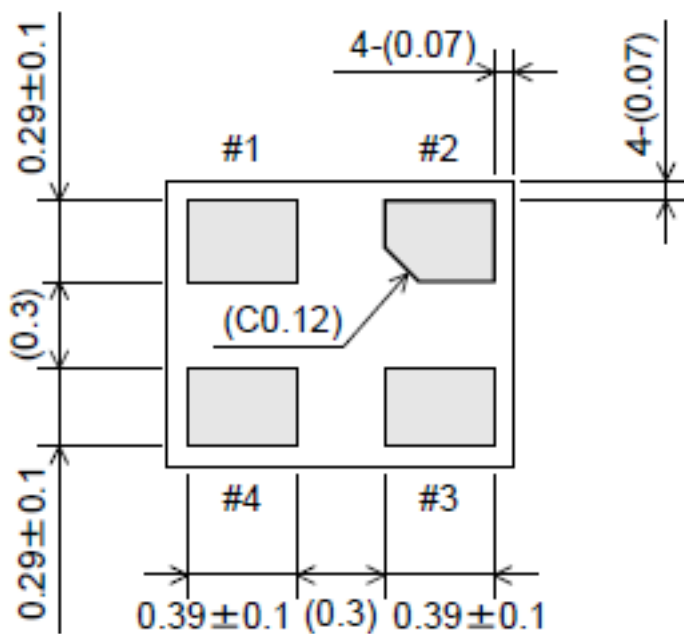
Bottom View
