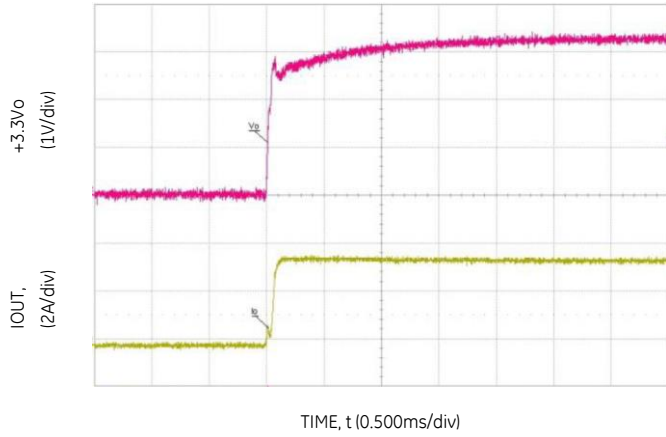
Fig 10: 3.3V Turn-On
