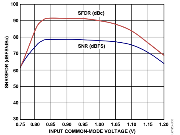
Figure 54. SNR/SFDR vs. Input Common Mode (VCM) with f_{IN} = 30 MHz
