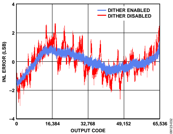
Figure 52. AD9268-125 INL with f_{IN} = 9.7 MHz
