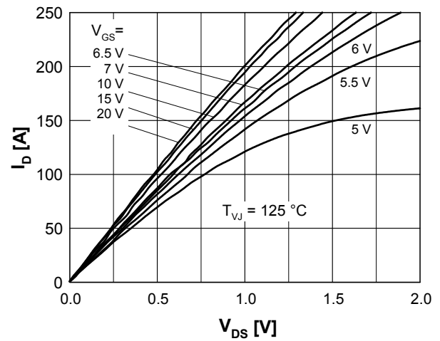
Fig. 4 Typ. output characteristics (125 ^{\circ}C )
