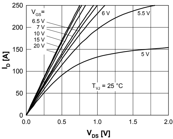
Fig. 3 Typ. output characteristics (25 ^{\circ}C )
