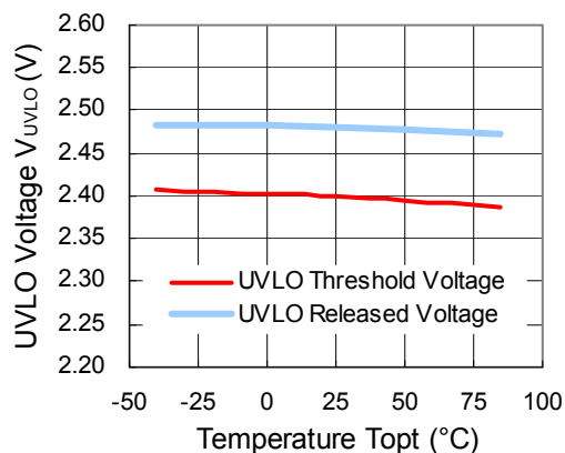
7) UVLO Voltage vs. Temperature
