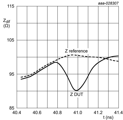
Fig. 5. Differential Time Domain Reflectometer (TDR) plot; typical values
