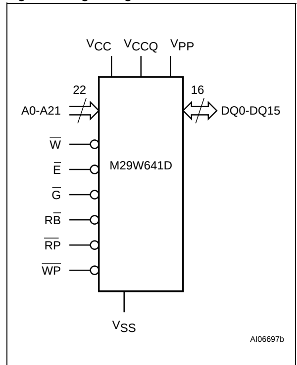
Figure 2. Logic Diagram
