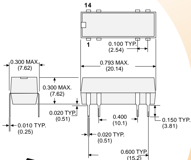
OUTLINE DIMENSIONS DIMENSIONS SHOWN IN INCHES & (MILLIMETERS).
