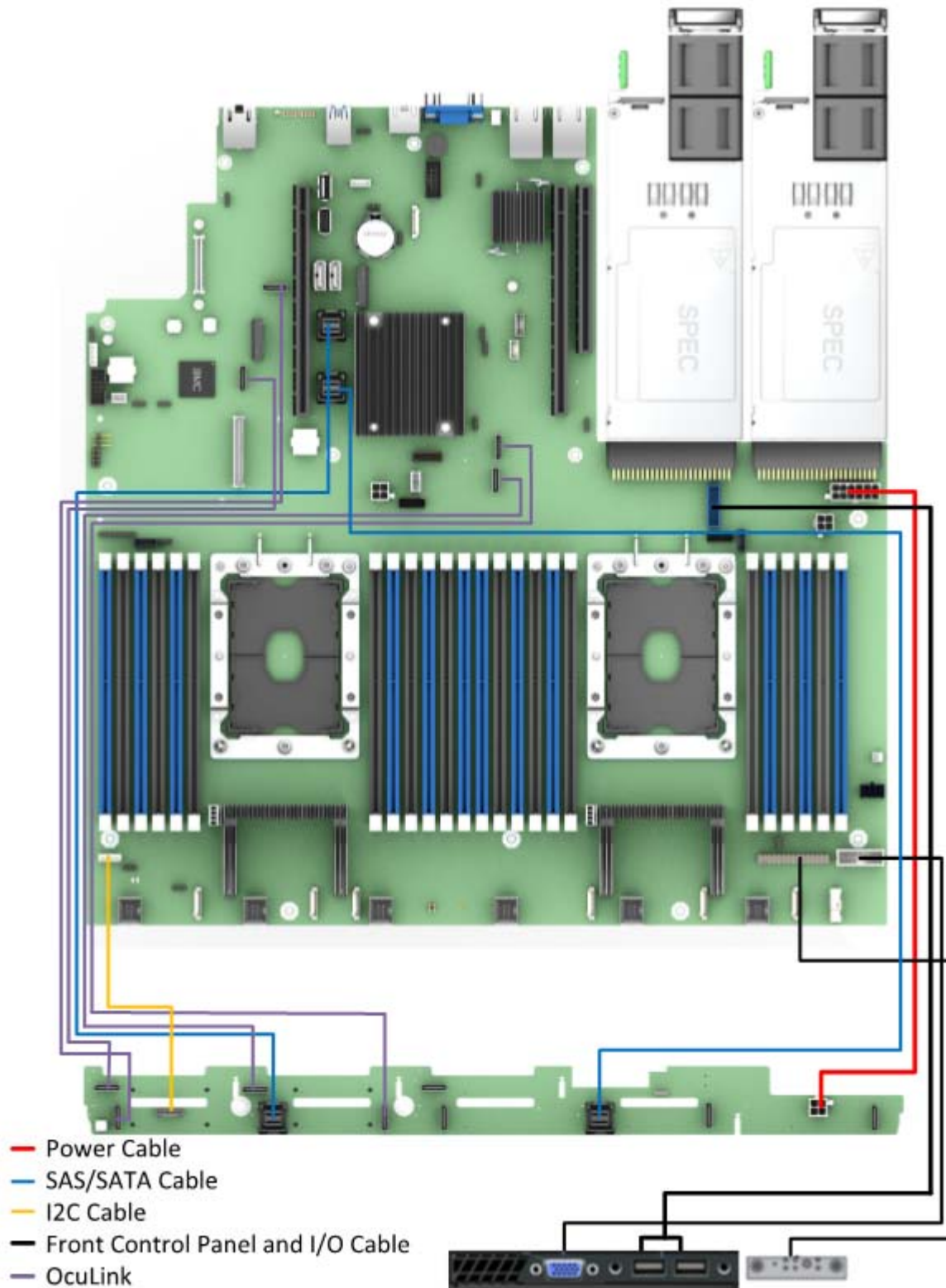
Figure 61. R1208WFxxx
