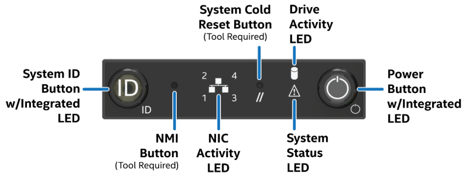
Figure 9. Front Control Panel Options
