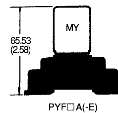
Mounting height of relay with socket
