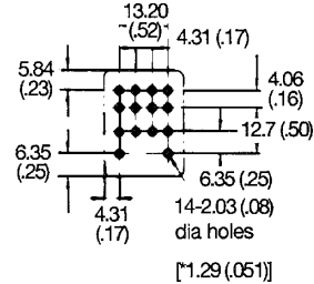
4PDT
