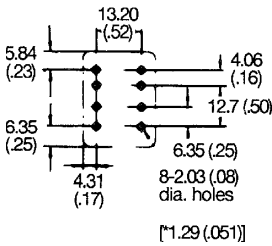
DPDT
