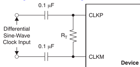
Figure 148. Differential Sine-Wave Clock Driving Circuit
