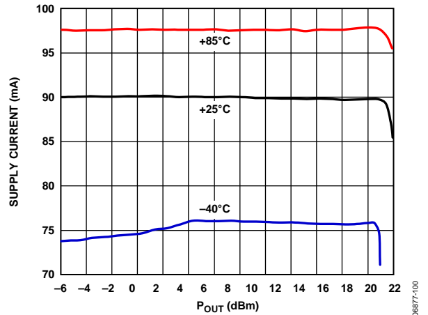
Figure 13. Supply Current vs. P OUT and Temperature
