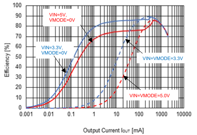
RP506Lxx1G/H/N V_{OUT} = 3.3\text{ V}
