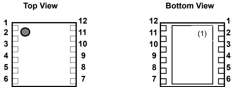
DFN3030-12 Pin Configurations
