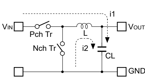
Basic Circuit
