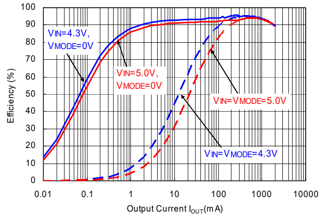
RP506Lxx1G/H/N V_{OUT} = 3.3\text{ V}
