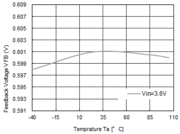
4) Feedback Voltage vs. Ambient Temperature RP506L001N/M
