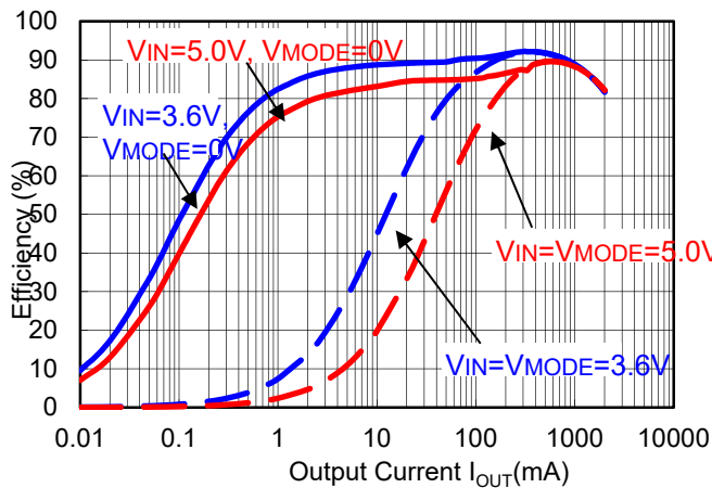
RP506Lxx1G/H/N V_{OUT} = 1.8\text{ V}
