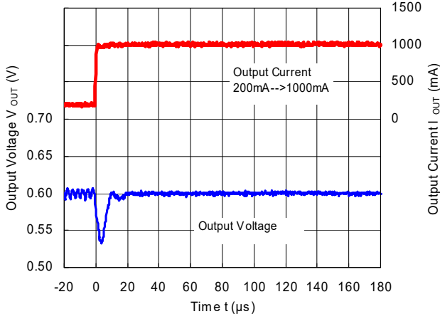
RP506Lxx1K/L/M ( V_{IN} = 3.6\text{ V} , V_{OUT} = 0.6\text{ V} ) MODE = "H" Forced PWM Control
