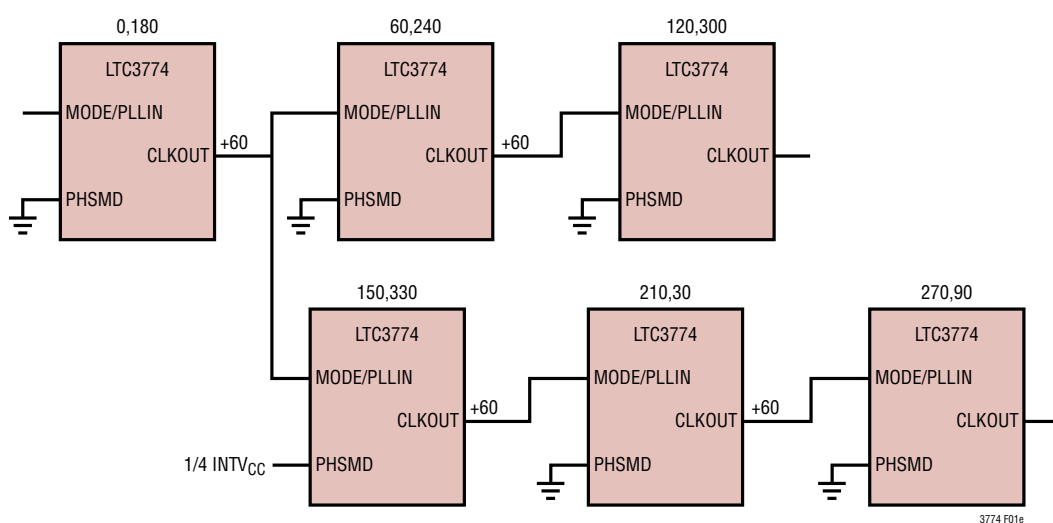
Figure 1e. 12-Phase Operation
