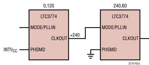
Figure 1a. 3-Phase Operation
