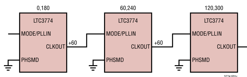
Figure 1c. 6-Phase Operation
