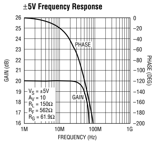
LT1253/54 • TPC15
