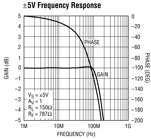
LT1253/54 • TPC11
