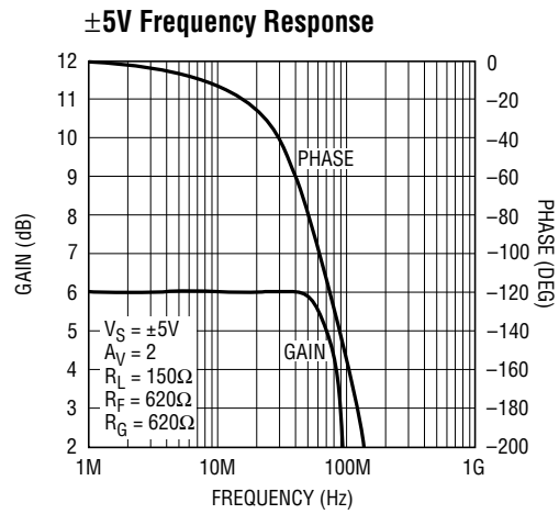
LT1253/54 • TPC13
