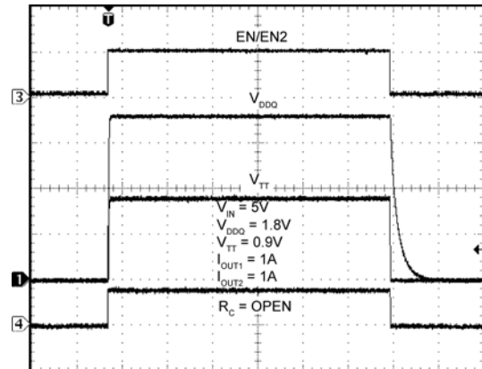
Time (4ms/div)
