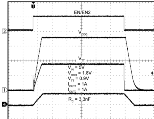
Time (4ms/div)
