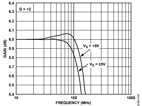
Figure 9. 0.1 dB Gain Flatness; V_S = +5 , V_S = \pm 5\text{ V}
