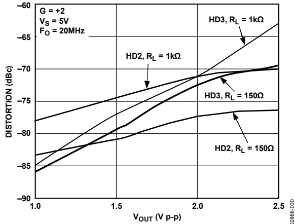
Figure 30. AD8007 Second and Third Harmonic Distortion vs. V_{OUT} and R_L
