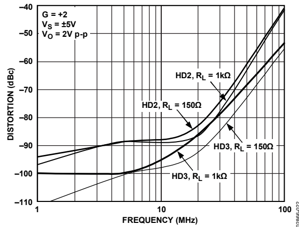
Figure 22. AD8007 Second and Third Harmonic Distortion vs. Frequency and R_L
