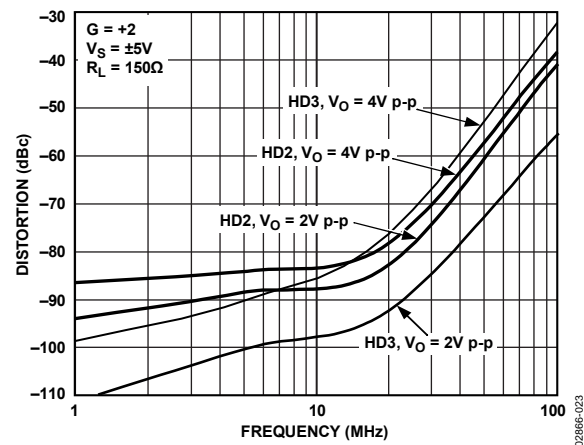
Figure 23. AD8007 Second and Third Harmonic Distortion vs. Frequency and V_O
