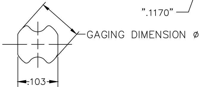
END VIEW OF DETAIL A (BOTH GAGE PINS)
