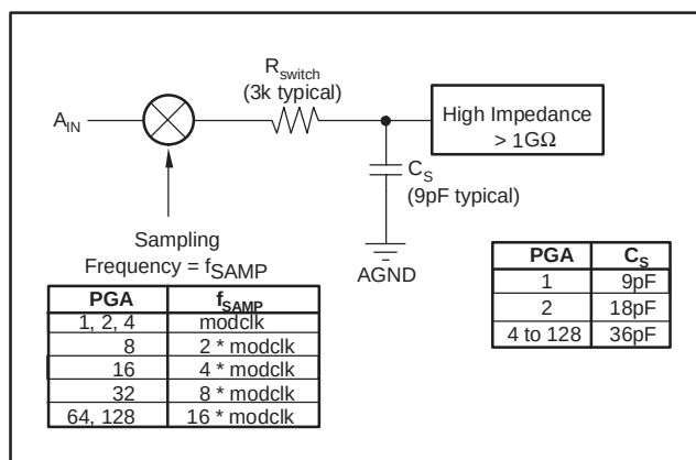
Figure 13. Analog Input Structure
