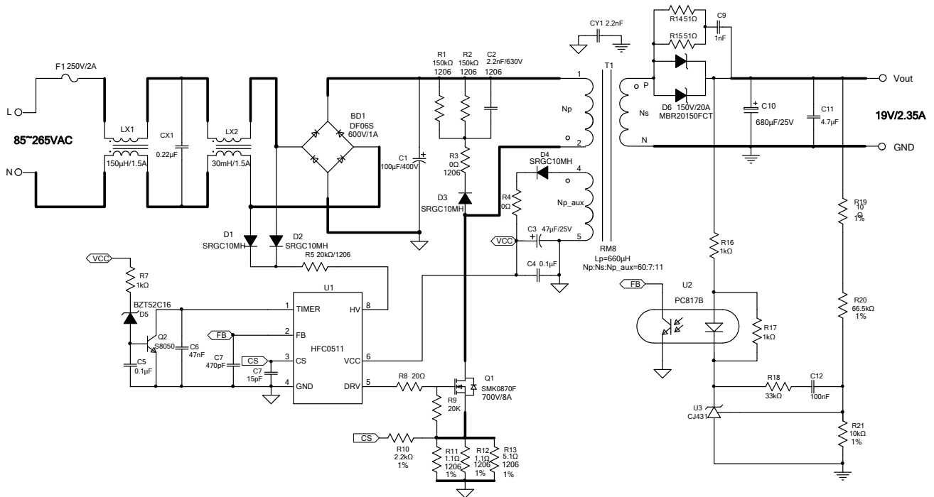
Figure 17: Typical Application
