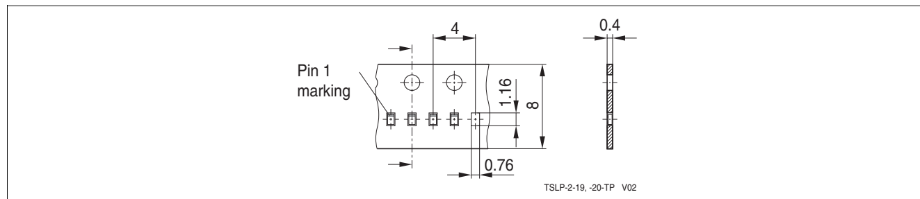
Figure 4-3 TSLP-2-19 Packing
