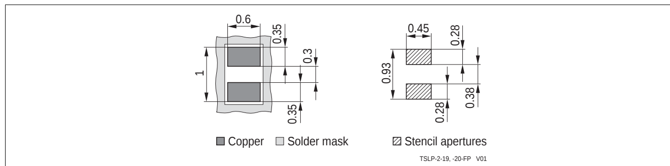
Figure 4-2 TSLP-2-19 Footprint
