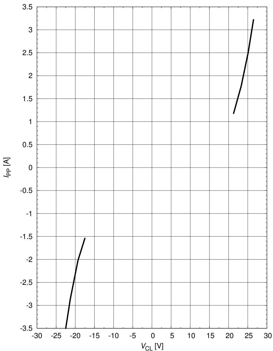
Figure 3-4 Clamping voltage(Surge): I_{PP} = f(V_{CL}) [1], pin 2 to pin 1
