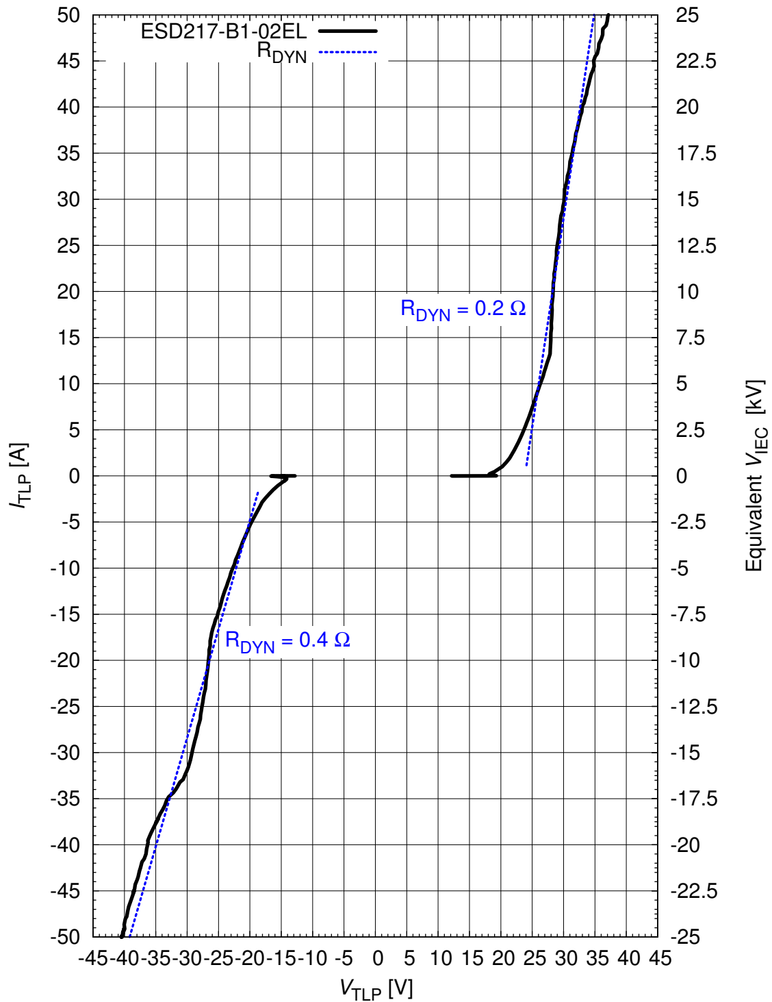
Figure 3-3 Clamping voltage (TLP): I_{TLP} = f(V_{TLP}) [1], pin 2 to pin 1
