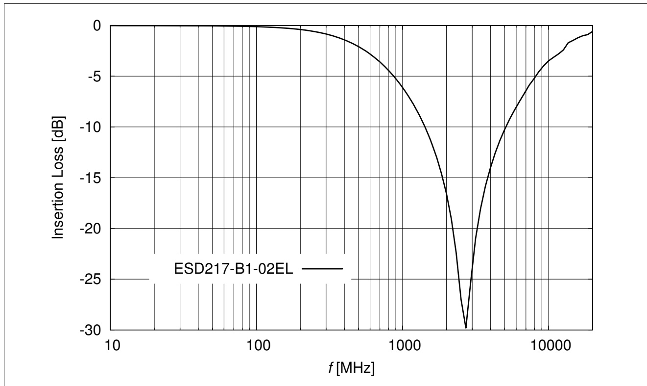
Figure 3-5 Insertion loss vs. frequency in a 50 \Omega system
