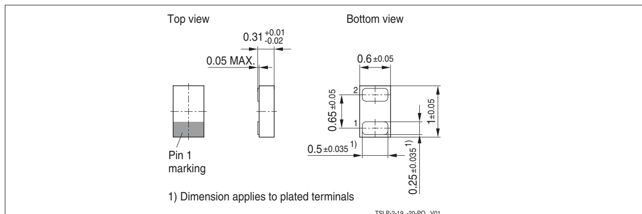
Figure 4-1 TSLP-2-19 Package outline
