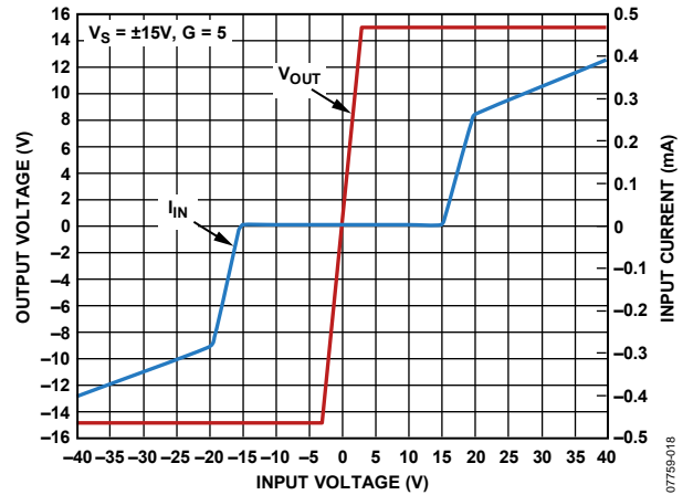
Figure 18. Input Overvoltage Performance, G = 5 , V_S = \pm 15 V
