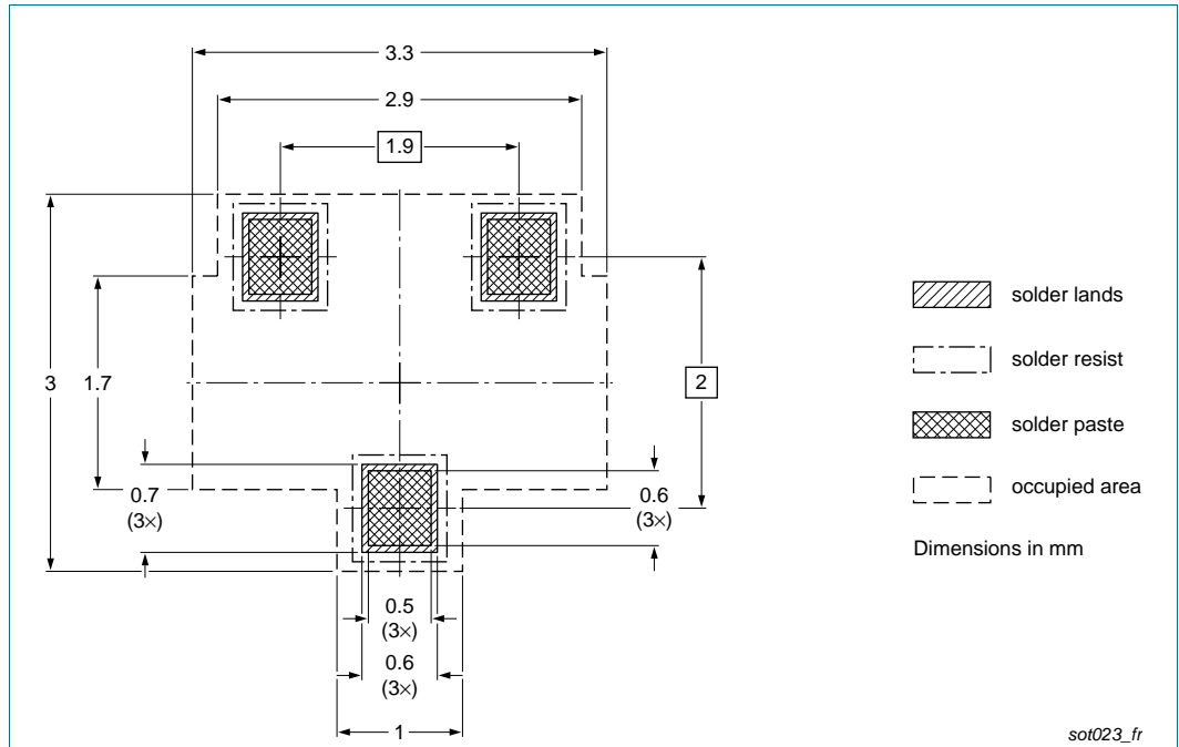
Dimensions in mm Fig 26. Reflow soldering footprint PDTD1xxxT series (SOT23/TO-236AB)
