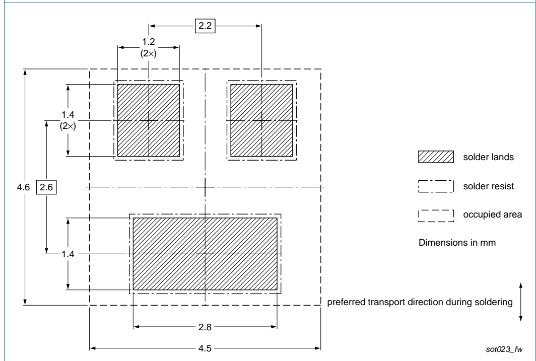
Dimensions in mm Fig 27. Wave soldering footprint PDTD1xxxT series (SOT23/TO-236AB)
