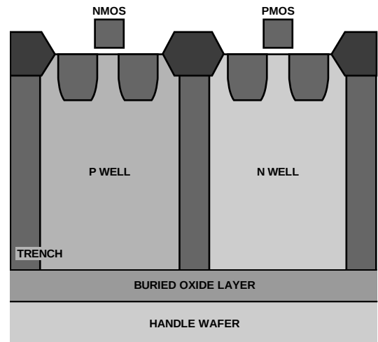
Figure 37. Trench Isolation
