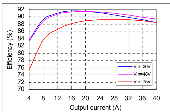
Figure 1 Efficiency vs. output current, Ta = 25°C, Vo = 1.8V, Air velocity = 300LFM
