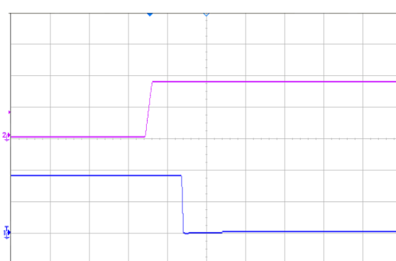
Figure 9 Output voltage shutdown by remote OFF, (20ms/div), see Figure 11 for test configuration; CH1-output voltage (1V/div); CH2-remote OFF voltage (2V/div) (Negative logic)
