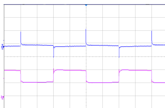
Figure 5 Dynamic response for 25% load step (25% ~ 50% ~ 25%) and 1A/µs slew rate, (2ms/div), see Figure 11 for test configuration; CH1-output voltage (50mV/div); CH2-output current (10A/div)
