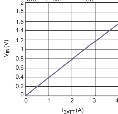
IB Voltage vs. Battery Current @ Boost Mode
