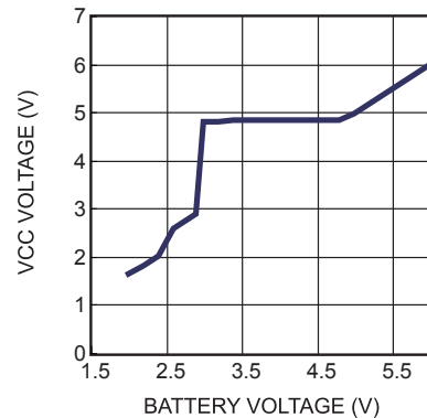
VCC @ Boost Mode
