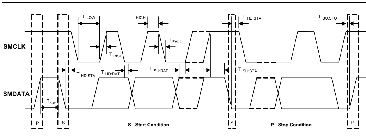
FIGURE 1-1: SMClock Timing.
