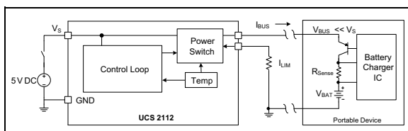
FIGURE 7-2: Constant Current Example.
