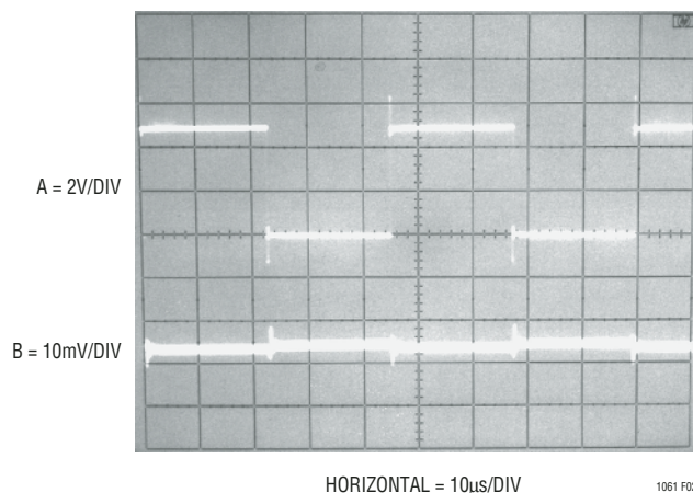
Figure 2. Typical Clock Feedthru of the LTC1061 Operating with \pm 5V Supplies. Top Trace is the Input Clock Swinging 0V to 5V and Bottom Trace is One of the Lowpass Outputs with Zero or DC Input Signals.
