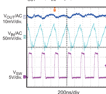
Input vs. Output Ripple
