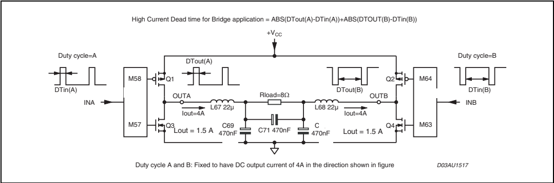
Figure 5. Test circuit
