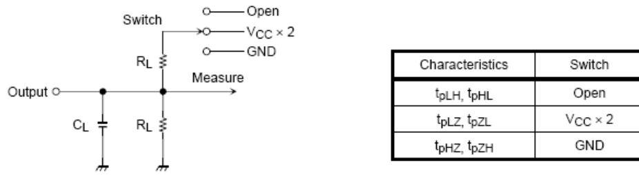
Figure 5. Test Circuit
