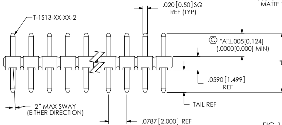
FIG 1 -S: SINGLE ROW OPTION MTMM-1XX-02-XX-S-100 SHOWN
