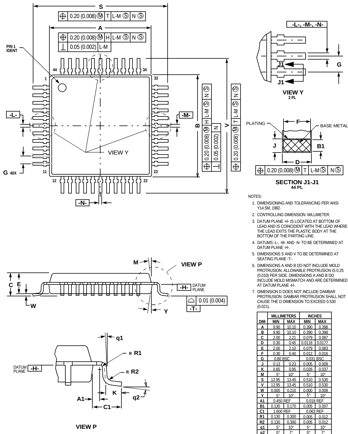
Figure 19-1. 44-Pin QFP (Case #824E)
