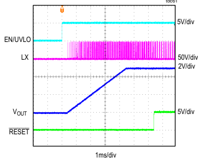
MAXM15063 STARTUP THROUGH ENABLE V_{IN} = 48V , FIXED V_{OUT} = 5V , FULL LOAD, PWM MODE
