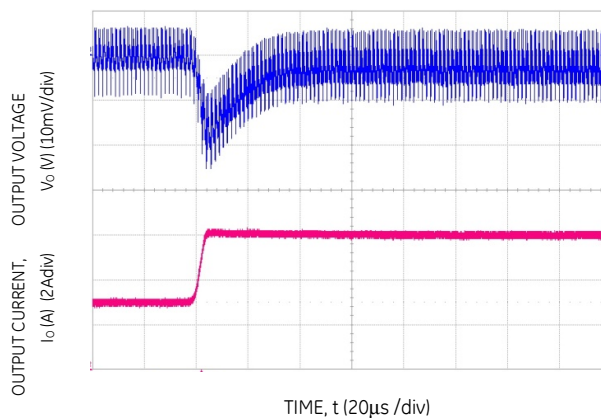
Figure 10. Transient Response to Dynamic Load Change from 50% to 100% at 12V in , C out =1x47μF+3x330μF, C Tune =12nF & R Tune =178
