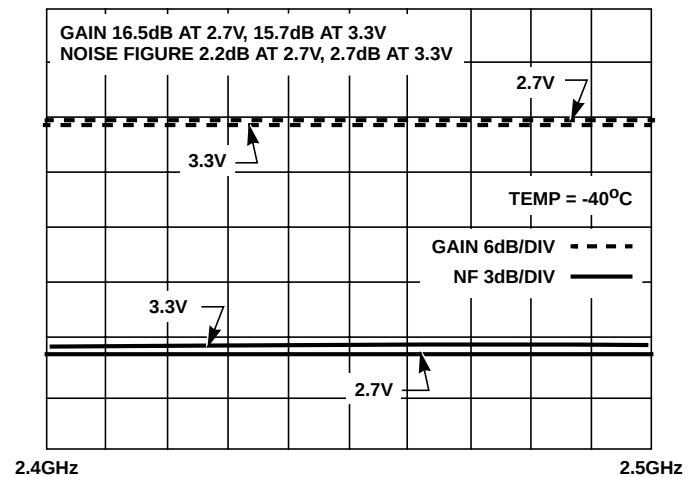
FIGURE 19. LNA HIGH GAIN AND NOISE FIGURE vs SUPPLY VOLTAGE
