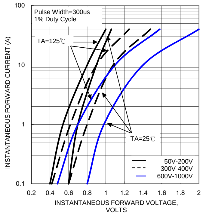
FIG. 5- TYPICAL INSTANTANEOUS FORWARD CHARACTERISTICS PER LEG
